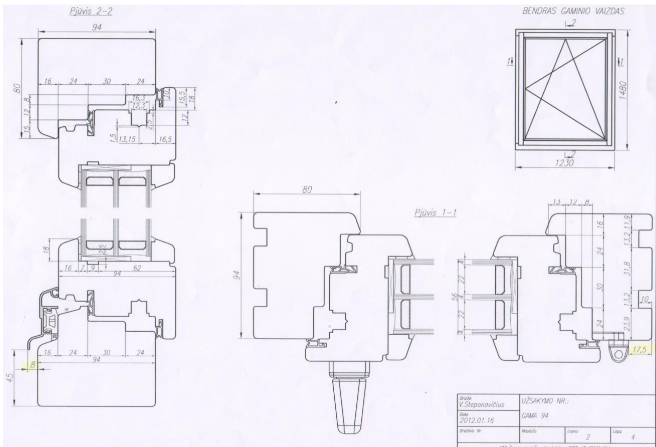
Fig 1. Window drawing (by the customer submitted information)
